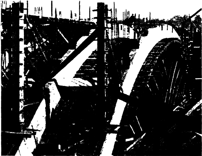
Fig. 297. —Timber Staging for Open-Spandrel Bridge.
